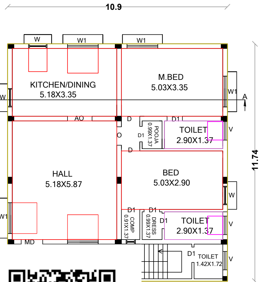
GR PLAN
