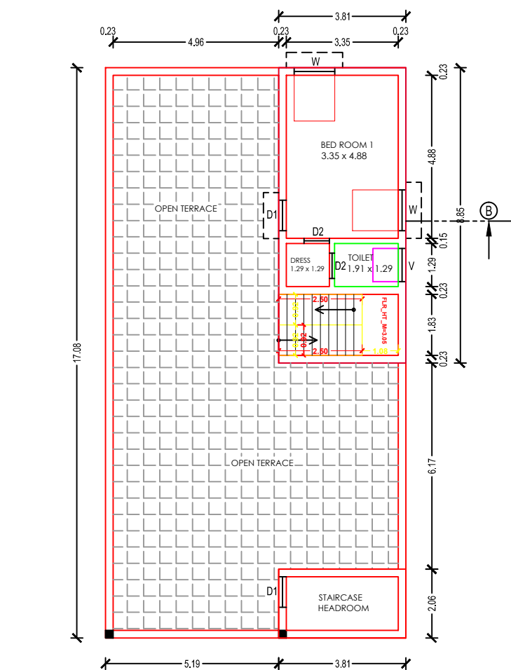
FIRST FLOOR PLAN ( BLOCK - 1 - PROPOSED RESIDENTIAL BUILDING )
