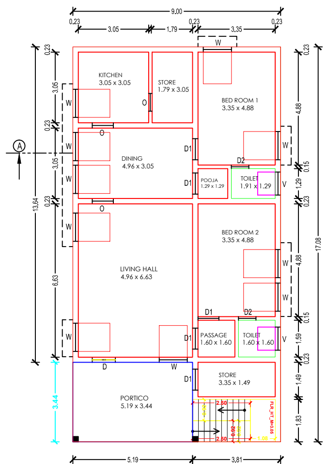
GROUND FLOOR PLAN ( BLOCK - 1 - PROPOSED RESIDENTIAL BUILDING )
