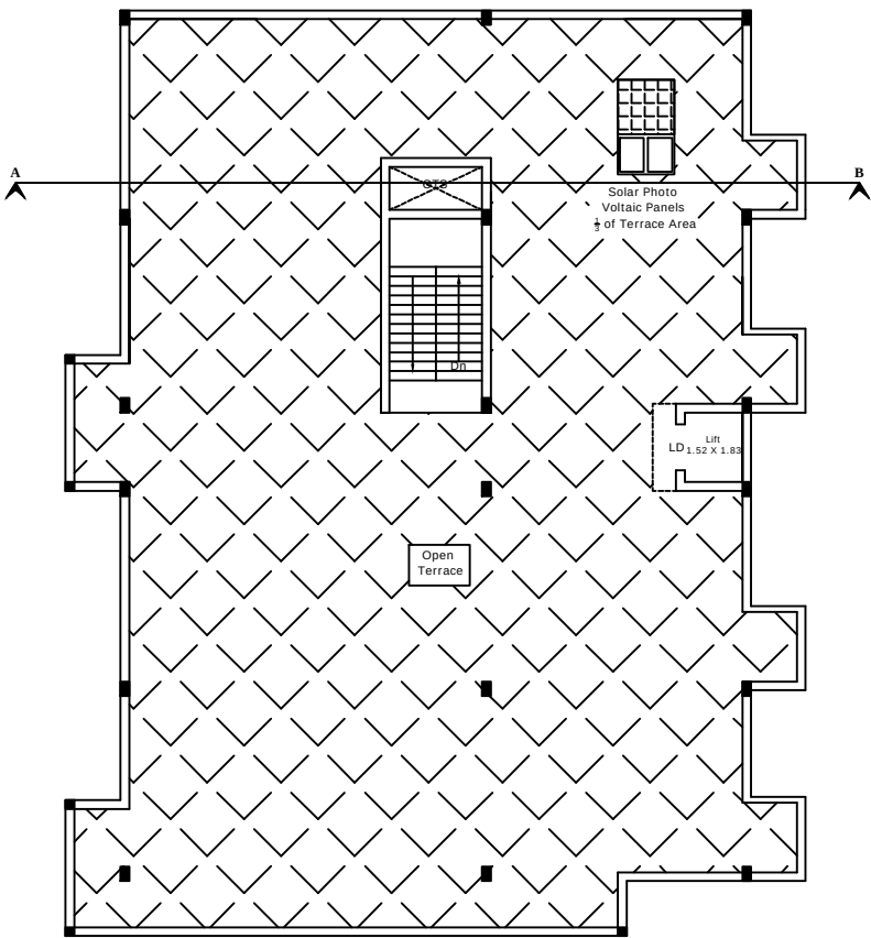
ROOF FLOOR PLAN SCALE - 1:100
