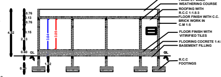
SECTION ON "S-S"
