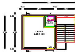
GROUND FLOOR PLAN (OFFICE ROOM)
