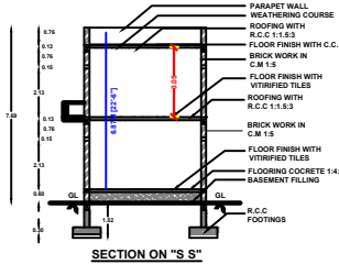
SECTION ON "S-S"
