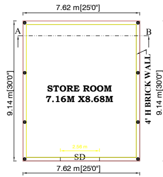
COMMERCIAL STORE - PLAN
