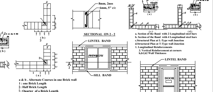
Figure - 3: Typical Details of Crossing Vertical Steel Bars in Brick Masonry.
