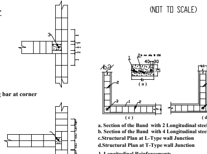
Figure - 2: Reinforcement and Bending Details of Section Bands.
