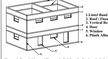
Figure - 1: Essential Internal Elements in Building for Earthquake Safety.
