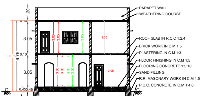
SECTION - XY
