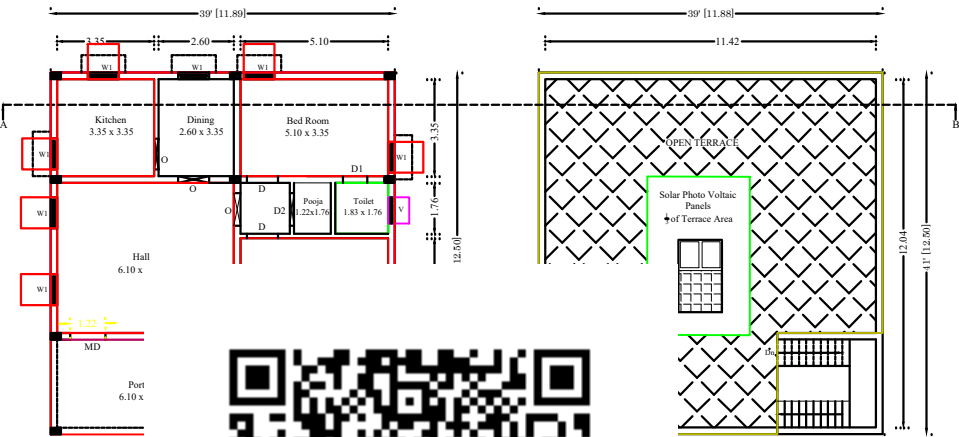
OOF FLOOR PLAN SCALE-1:100
