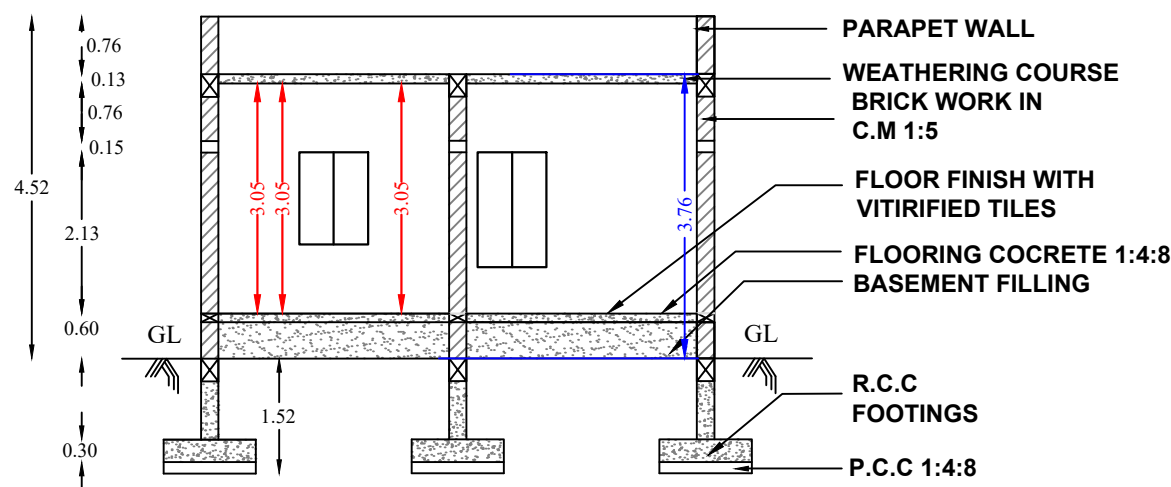
SECTION ON "S S"
