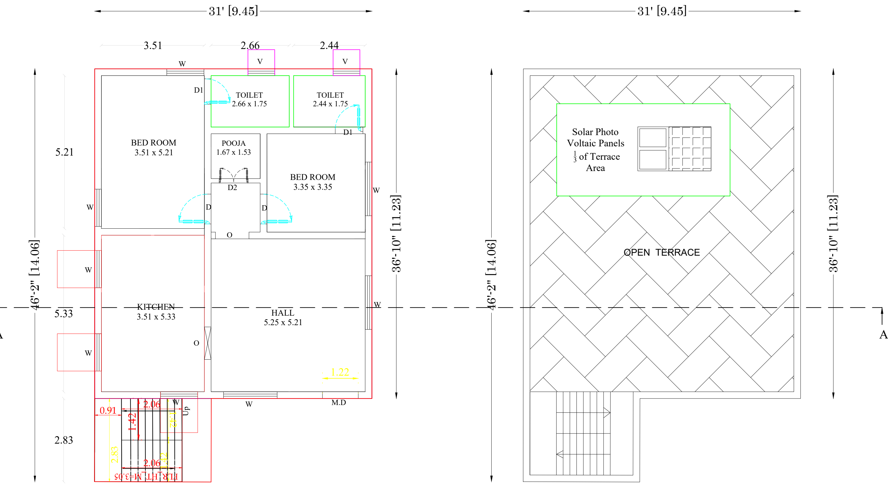
ROOF FLOOR PLAN SCALE - 1:100
