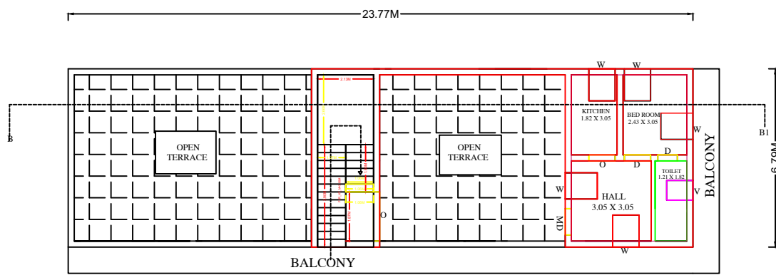
FIRST FLOOR
