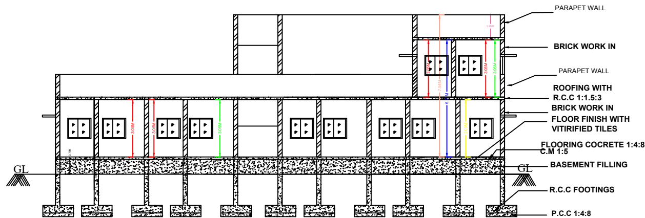
SECTION AT B-B1
