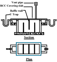
Using "U" type trap 2 Nos in inter. outlet & Ventpipe will be covered with mosquito proof covering net in inner side of vent pipe and top of vent pipe. Septic Tank With U Trap Not To Scale
