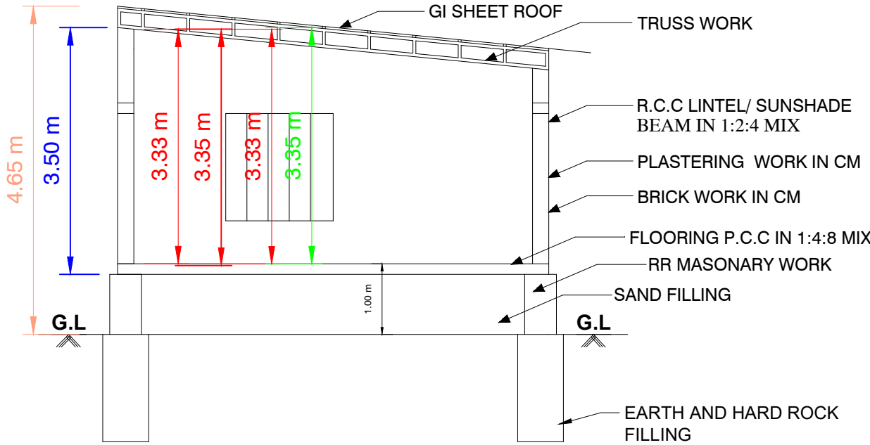
SECTION"AB"
