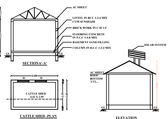
CATTLE SHED-PLAN
