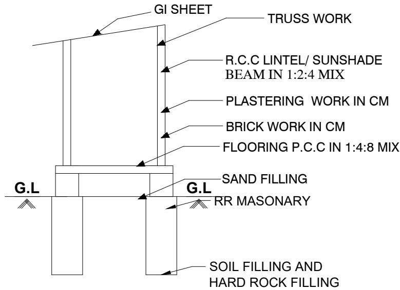
SECTION"AB"
