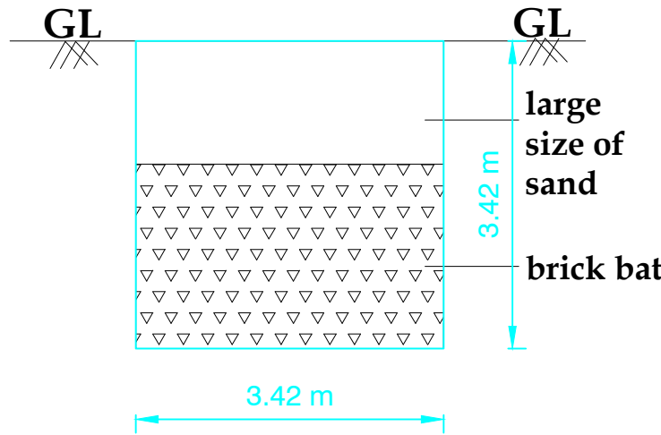
RAINWATER HARVESTING
