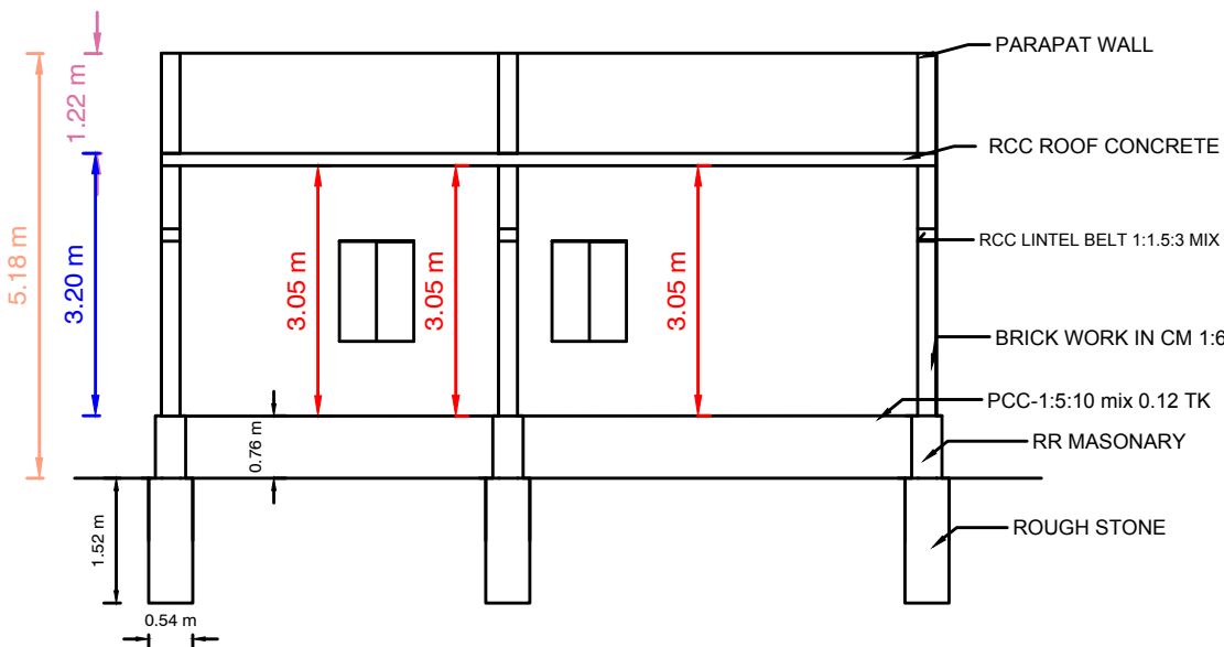
SECTION"AB"
