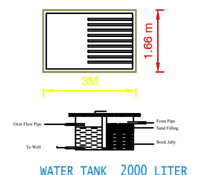
WATER TANK _2000 LITER
