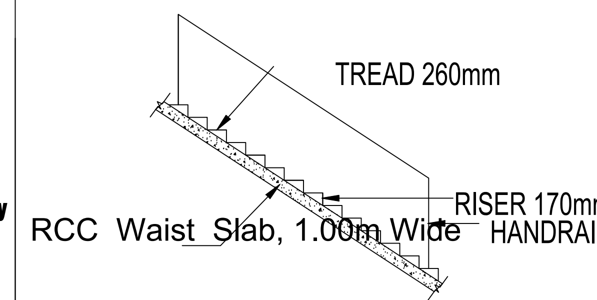
STAIRCASE DETAILS
