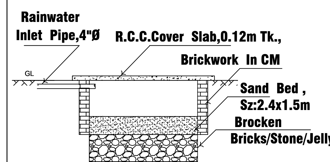
SECTION ON "MN"
