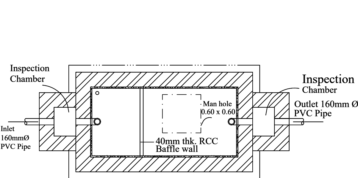
septic tank
