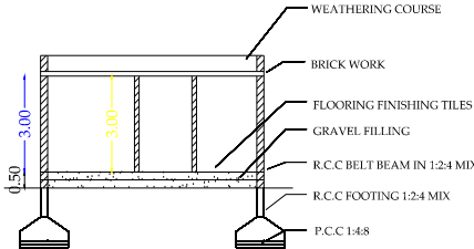
SECTION A TO B
