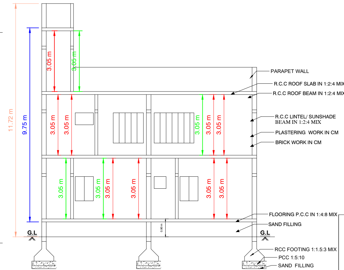
SECTION"AB"
