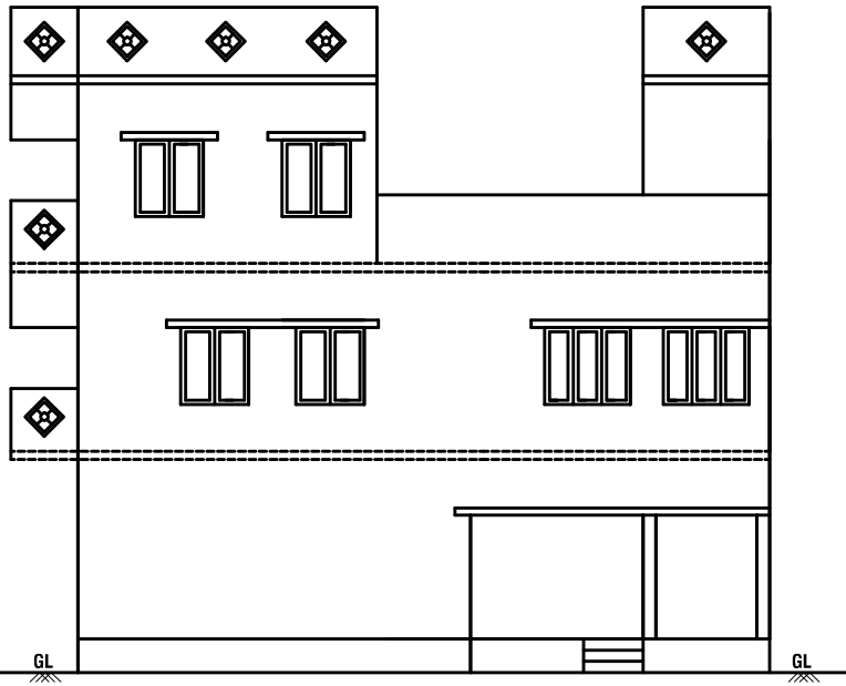
ELEVATION ( FROM EAST )
