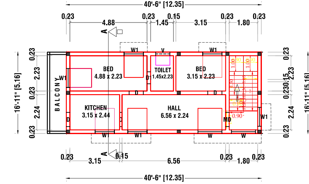
FIRST FLOOR PLAN ( PROPOSED CONSTRUCTION )
