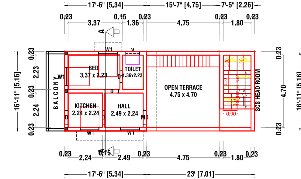
SECOND FLOOR PLAN ( PROPOSED CONSTRUCTION )
