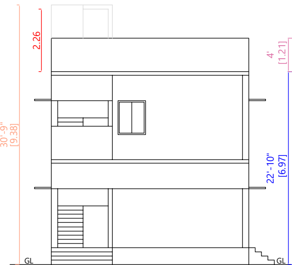
FRONT ELEVATION (WEST SIDE VIEW)
