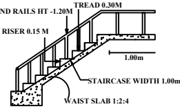
STAIRCASE DETAILS
