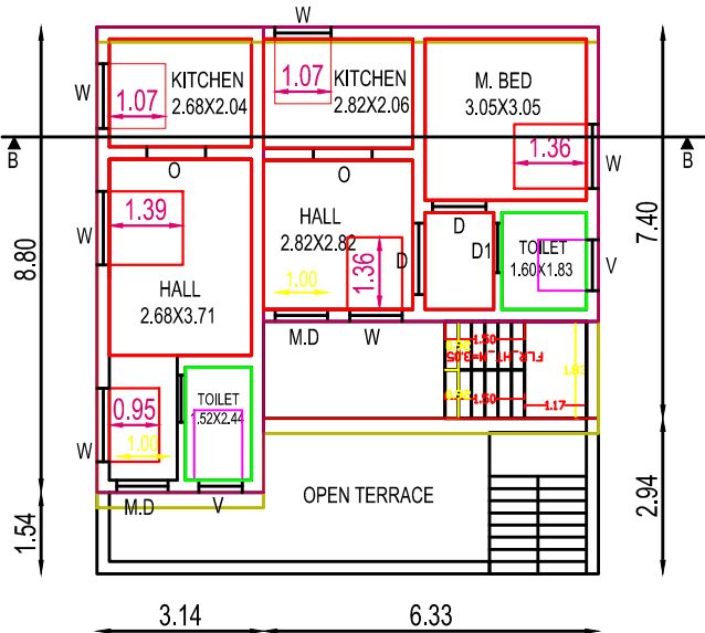
FIRST FLOOR PLAN (PROPOSED BUILDING)
