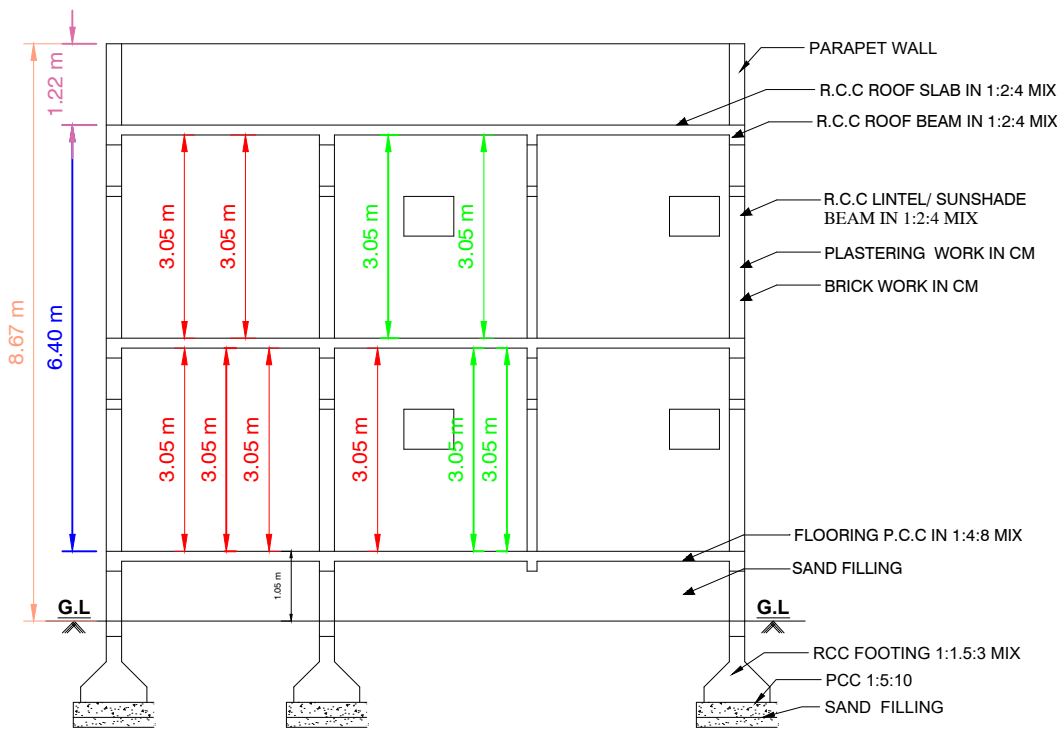
SECTION"AB"
