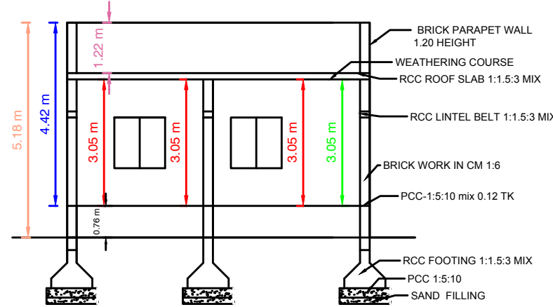
SECTION " AB "
