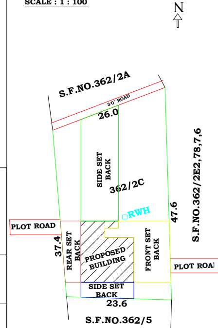
RAINWATER HARVESTING RW TANK CAPACITY=2000LITER
