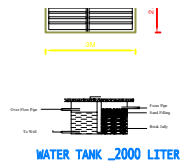
WATER TANK _2000 LITER
