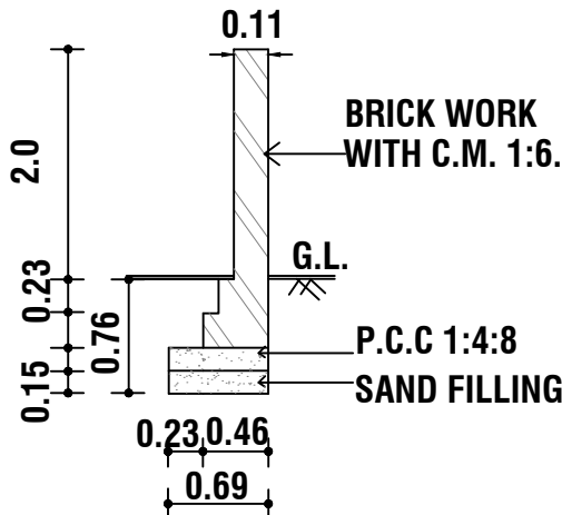
SECTION OF COMPOUND WALL
