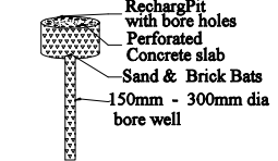
RAIN WATER HARVESTING
