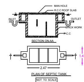
PLAN OF SEPTIC NOT TO SCALE
