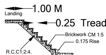
Staircase Details.
