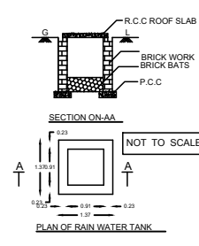
1.37 PLAN OF RAIN WATER TANK
