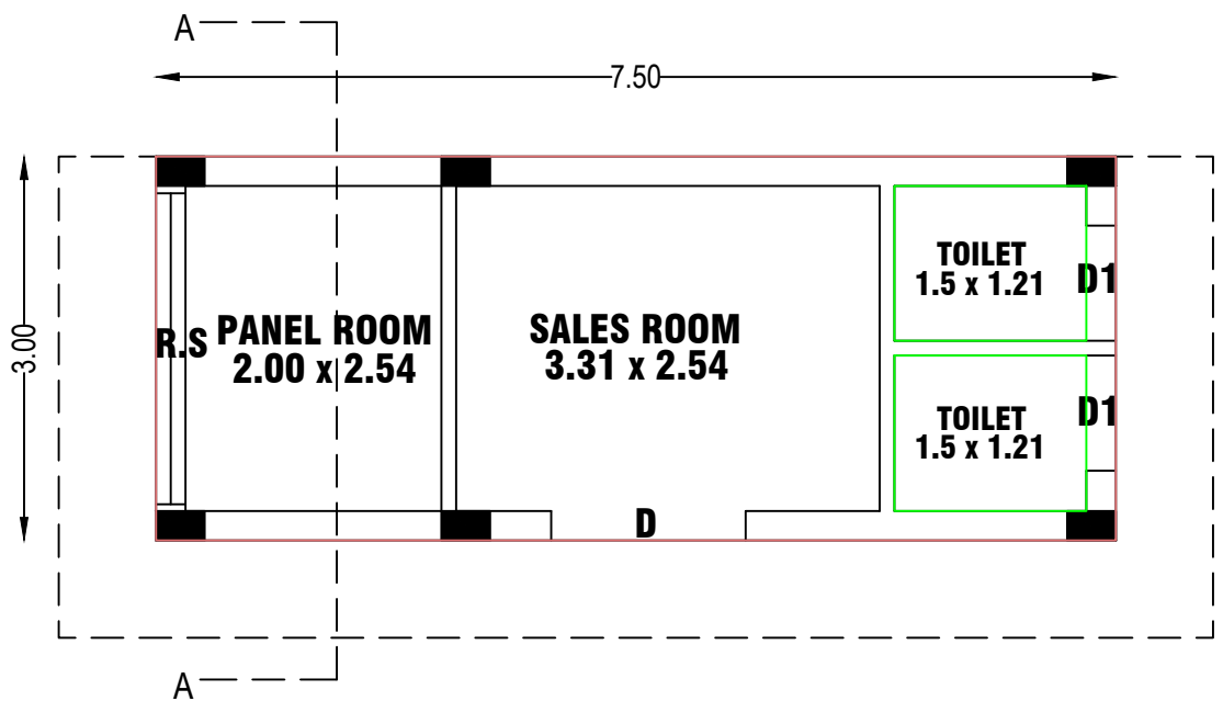
PLAN (SCALE 1:100)
