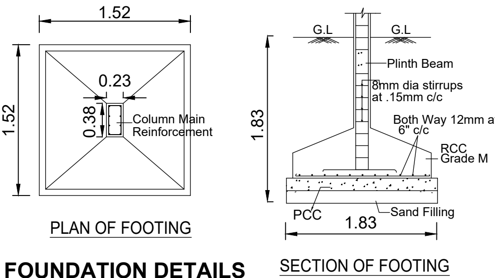
FOUNDATION DETAILS
