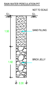
RAIN WATER PERCOLATION PIT
