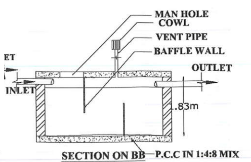
SECTION ON BB - P.C.C IN 1:4:8 MIX
