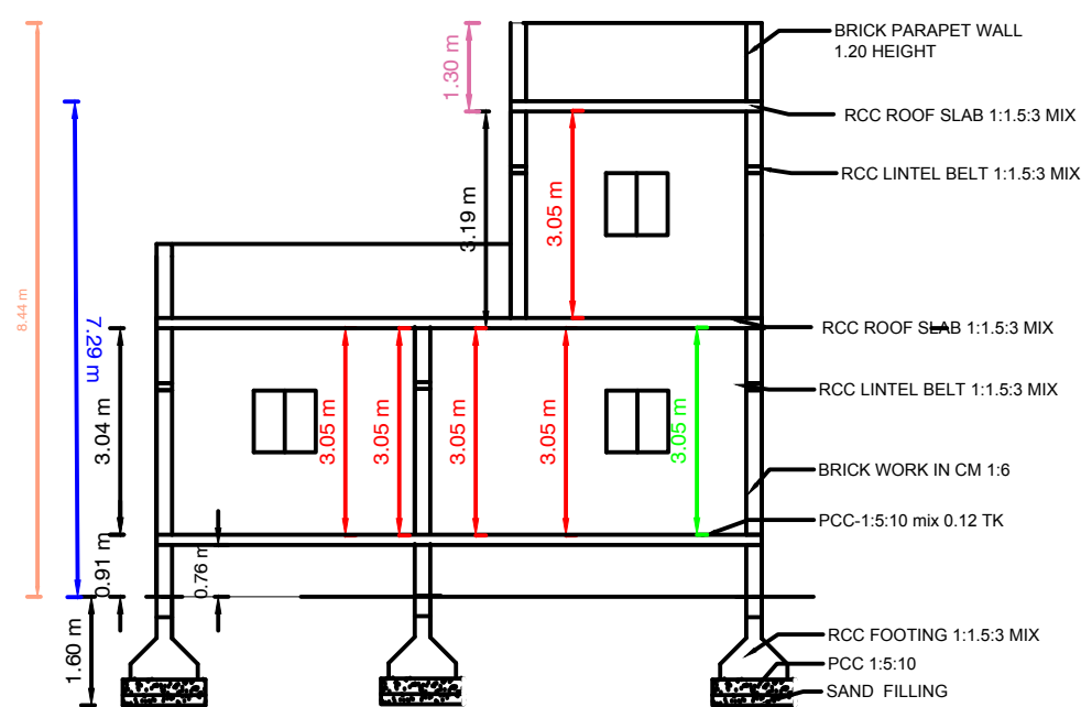
SECTION "AB"
