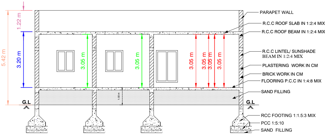
SECTION"AB"
