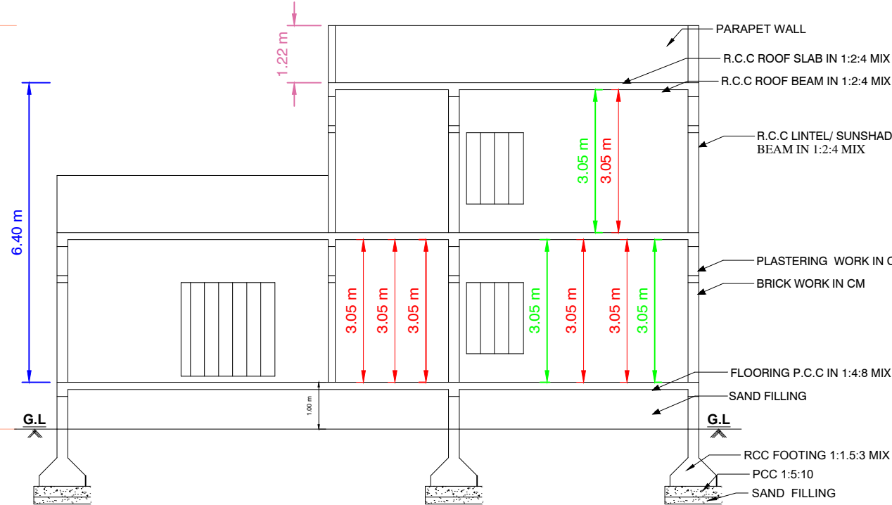
SECTION"AB"
