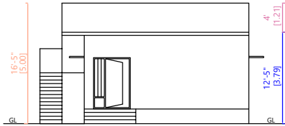
FRONT ELEVATION (NORTH SIDE VIEW)
