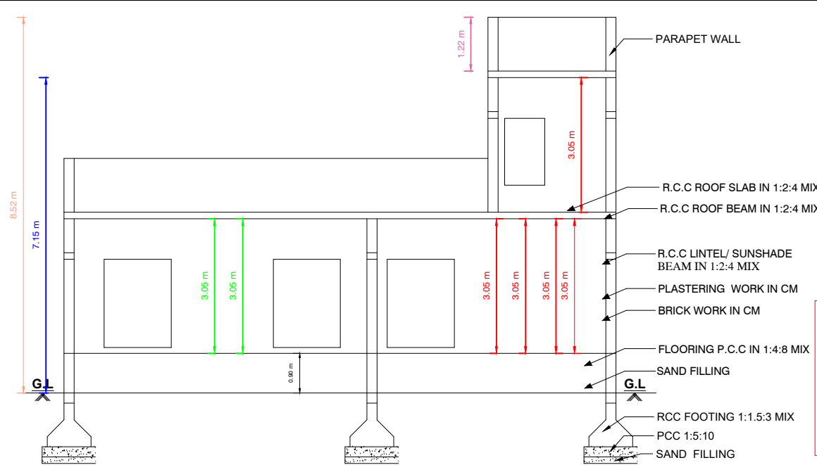
SECTION "AB"
