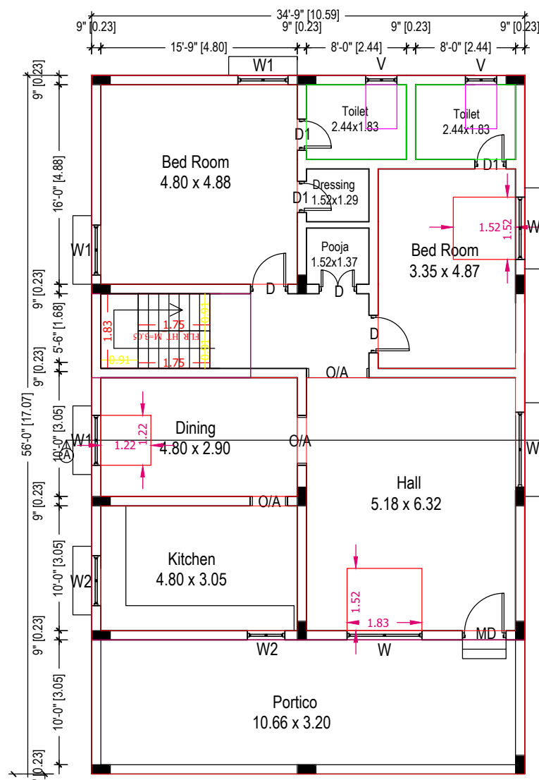
EXI.GROUND FLOOR PLAN
