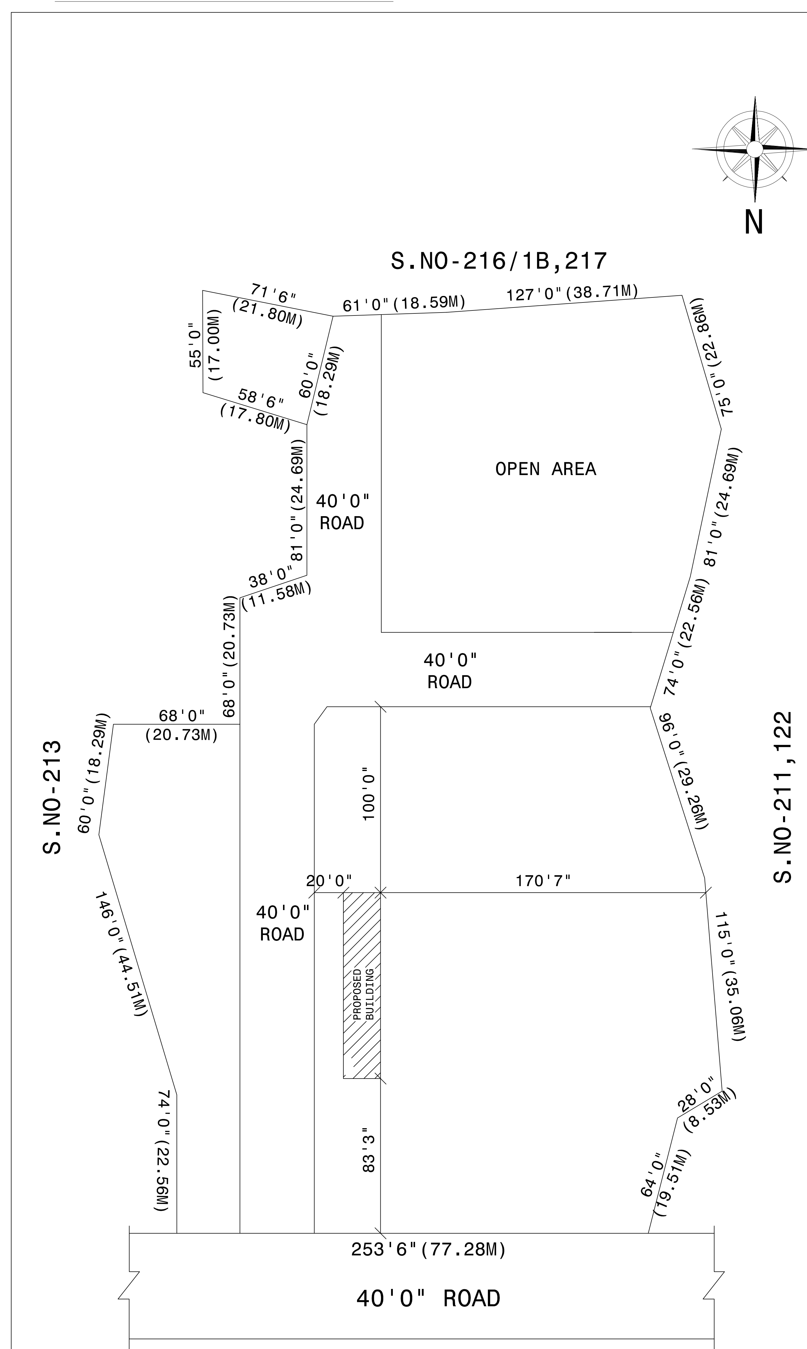
SITE PLAN NOT TO SCALE
