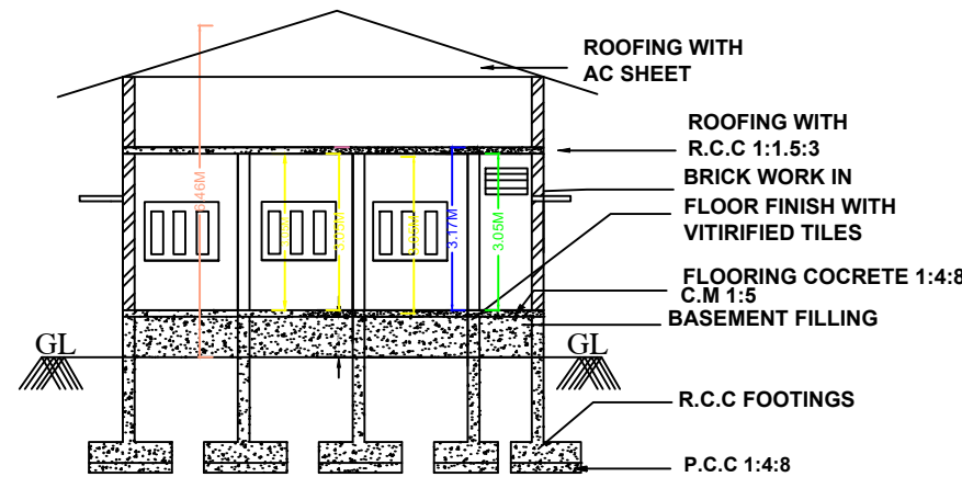
SECTION ON "BB1"
