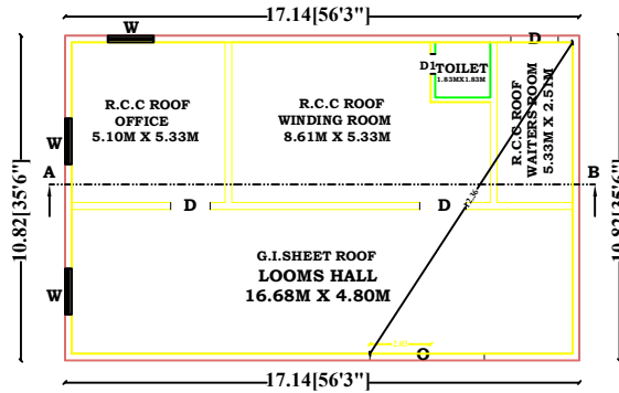
LOOMS BUILDING - PLAN [PART-I]
