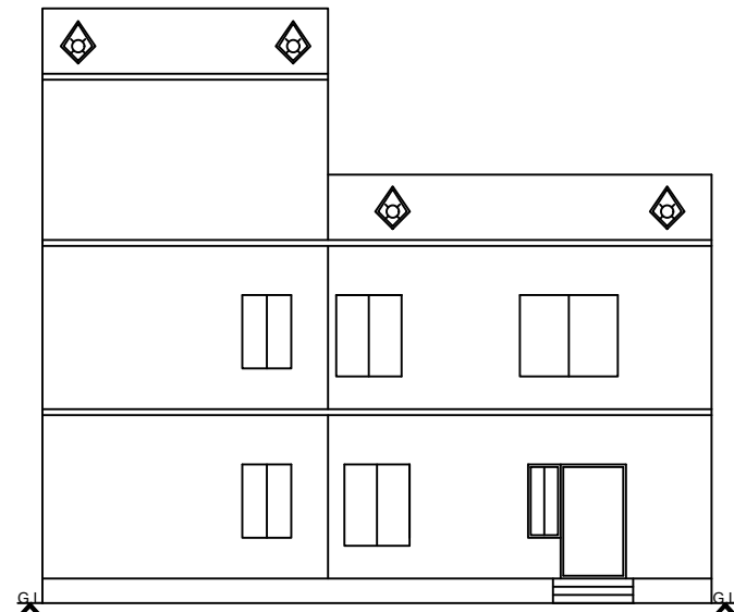
FRONT ELEVATION
