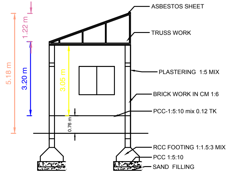
SECTION"AB"
