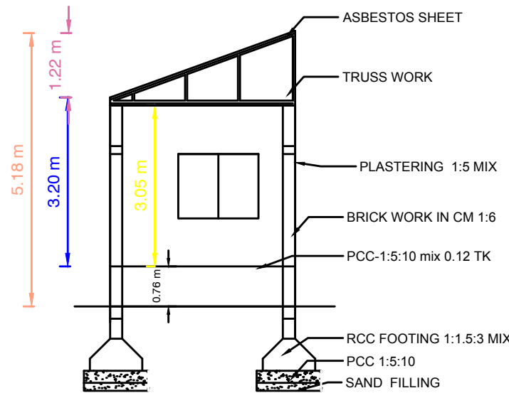
SECTION"AB"
