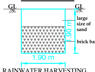
Septic Tank With U Trap Not To Scale
