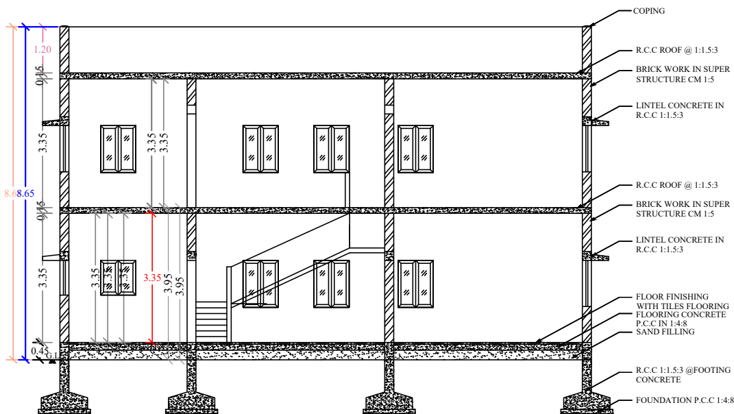
SECTION-AB
