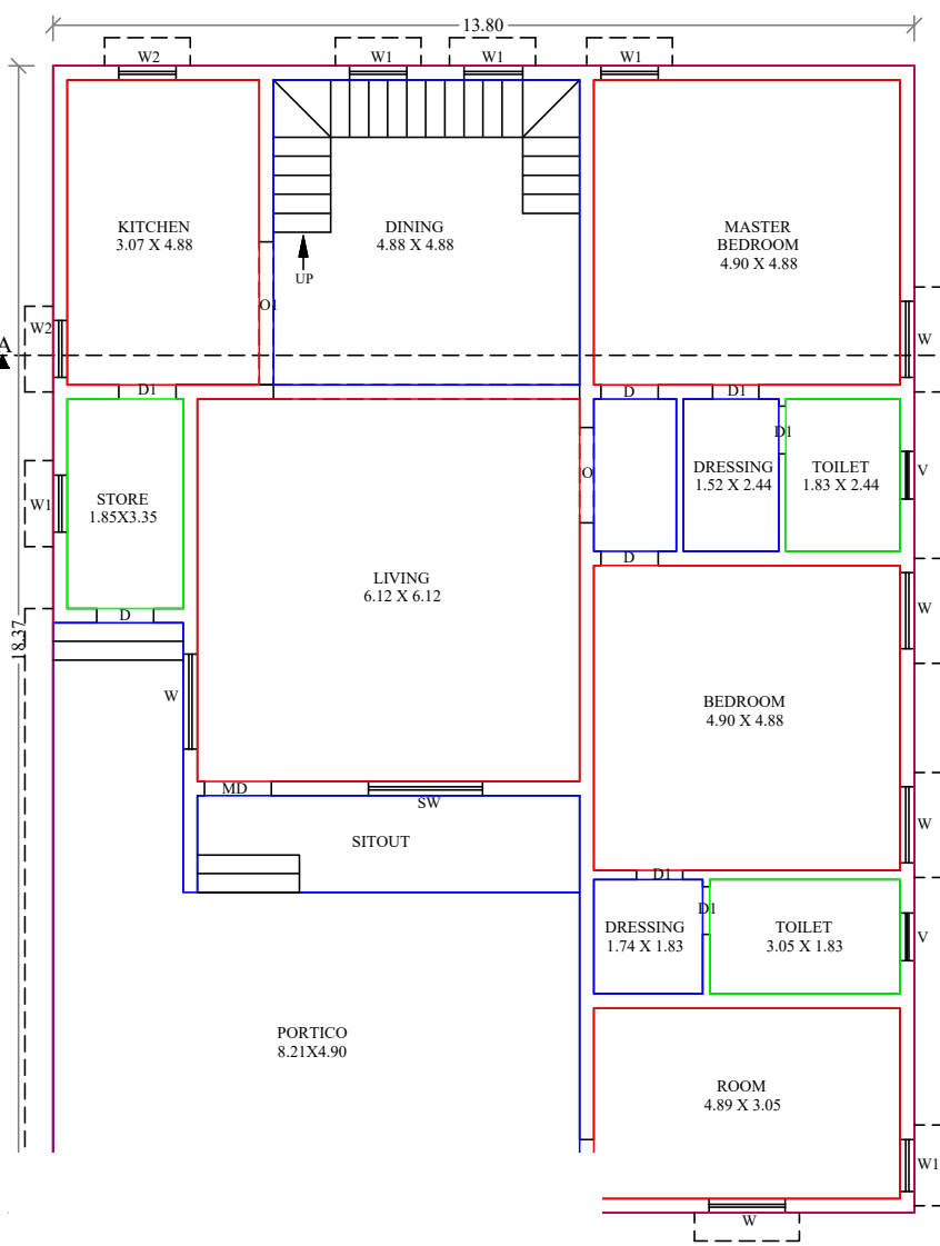
FLOOR PLAN
