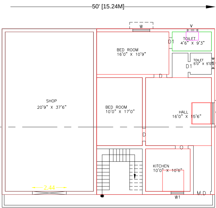
PLAN - FIRST FLOOR
