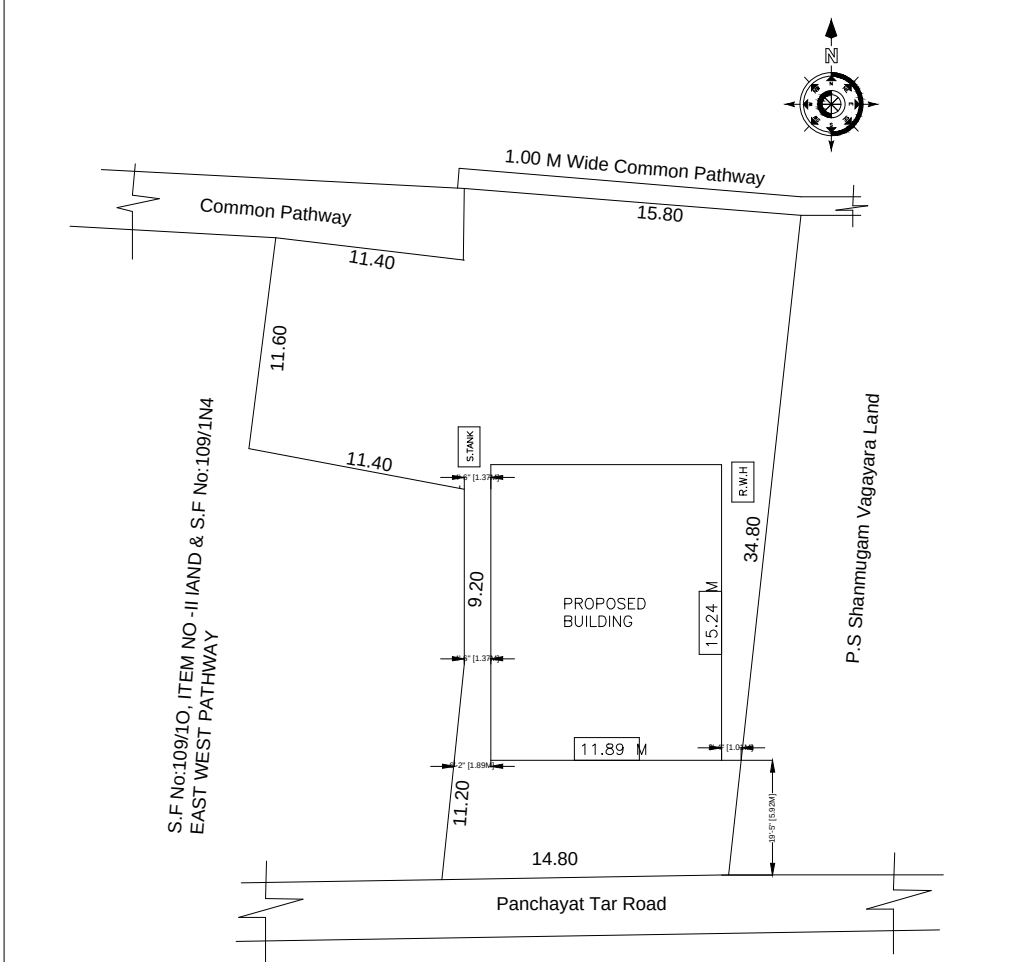
SITE PLAN
