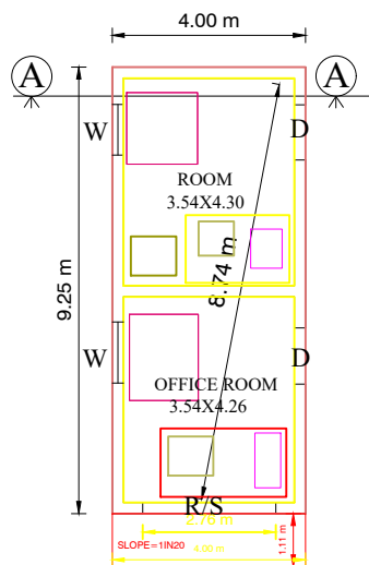
PROPOSED GROUND FLOOR
