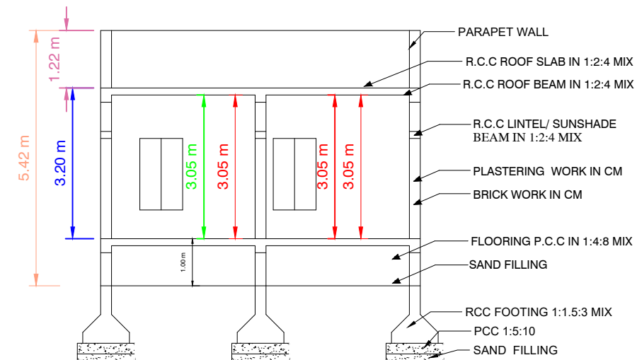
SECTION"AB"
