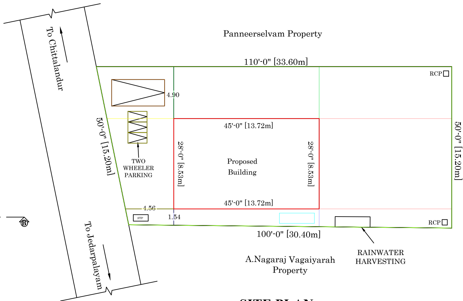
SITE PLAN
