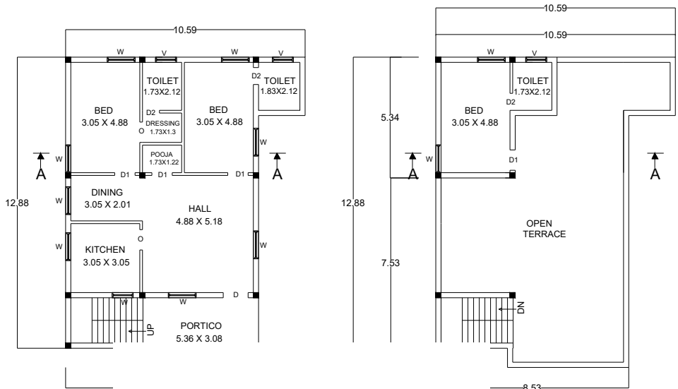
1ST FLOOR PLAN SCALE- 1:100
